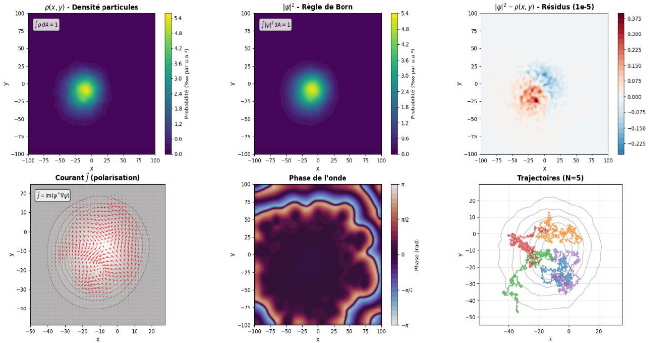
Fig 3. Simulation 2D. (Top) Comparison between particle density and Born's rule. (Bottom-left) Probability current vectors showing the internal field dynamics.
